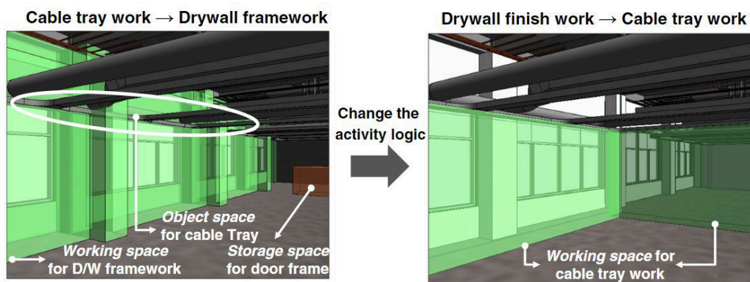
Figure 4. Workspace problem identification and resolution
