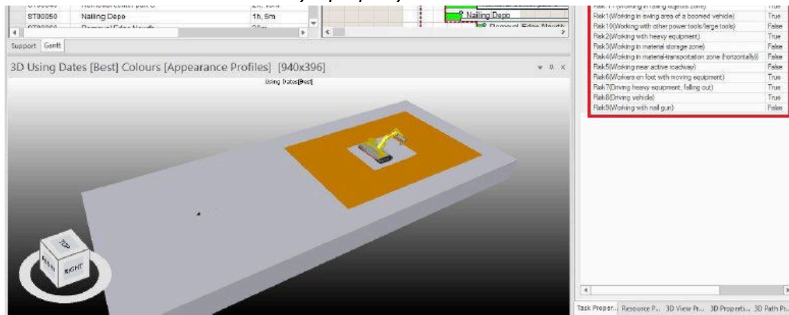
Figure 3. A view of a project's 4D BIM model representing the presence or absence of the hazardous attributes in the activity's property menu
