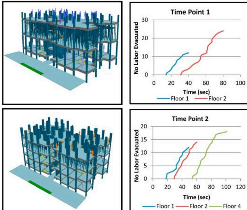
Figure 7. BIM model over time alongside evacuation time
